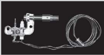
Series 15 ODS assembly
