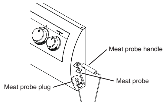
Fig. 21-1 Meat probe detail
