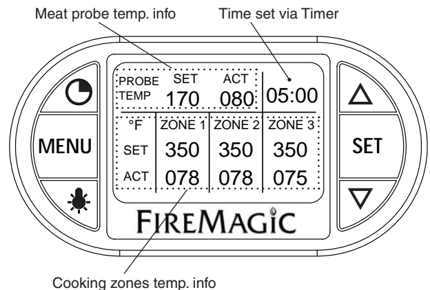
Fig. 21-3 Default screen detail
